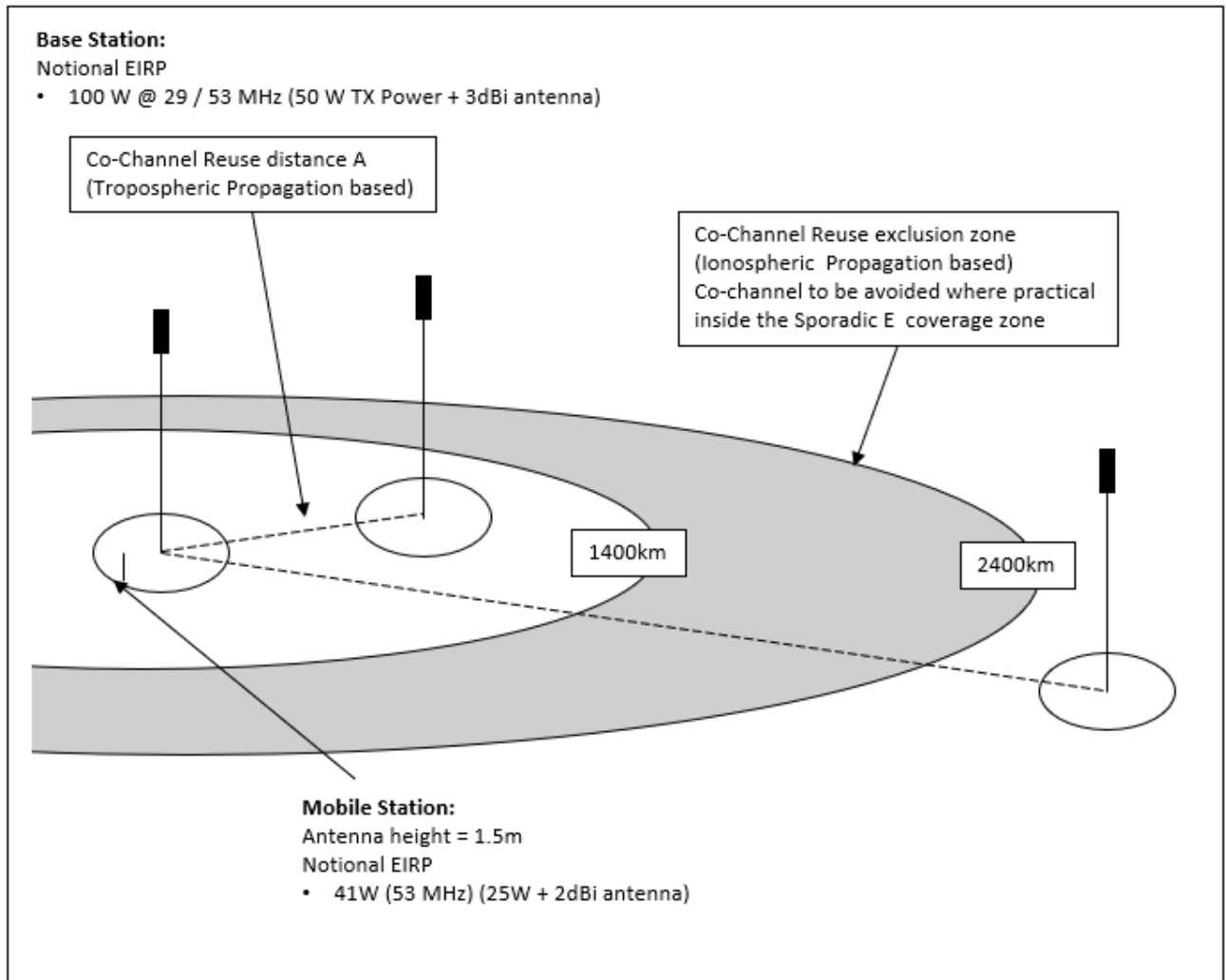
Figure – Amateur Repeater Model < 100 MHz
